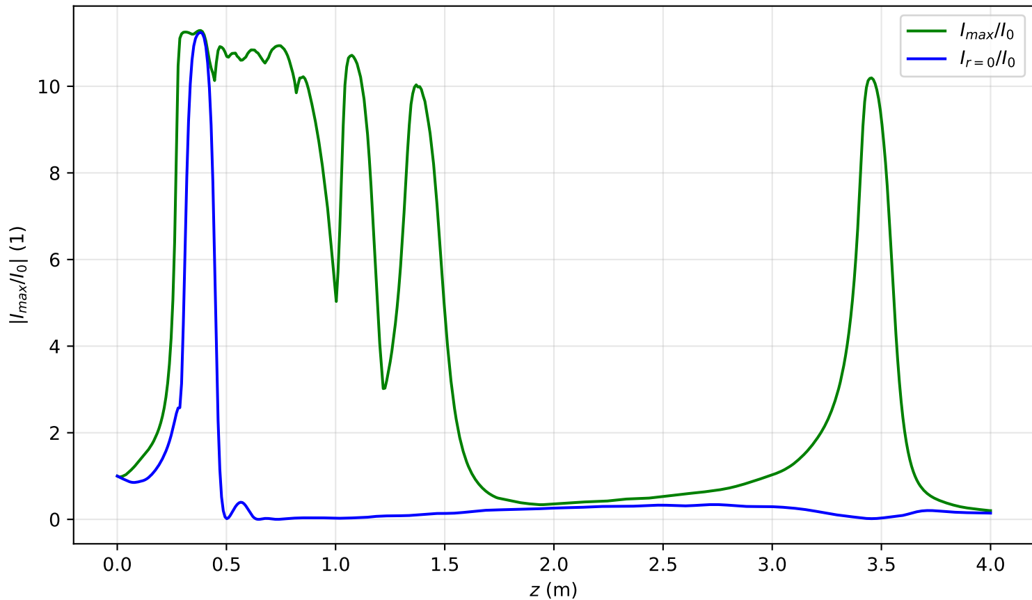
I_{max}(x = 0, y = 0, z)/I_0 , Pin=9.8Pcr, noisy input, artificial time
